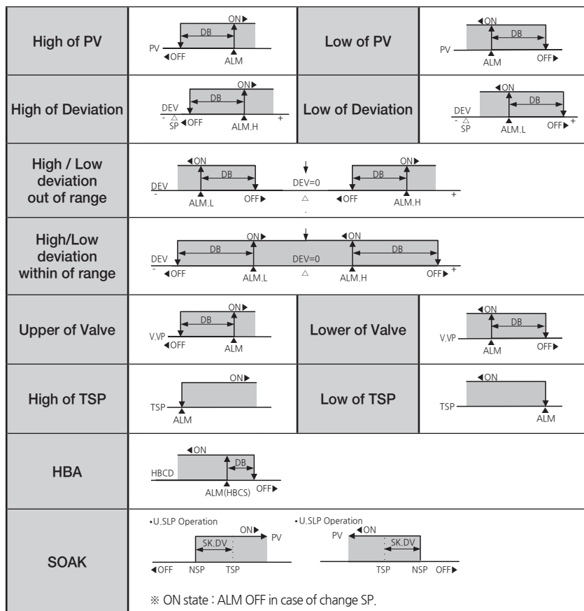
[Fig.27] Alarm Operation
