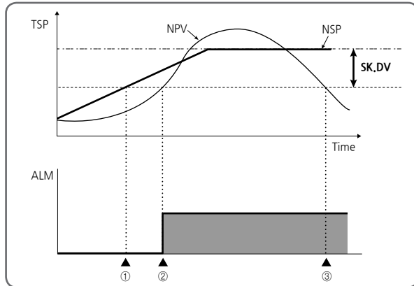
[Fig.28] UP SLOPE(∧ : SP ramping up)
