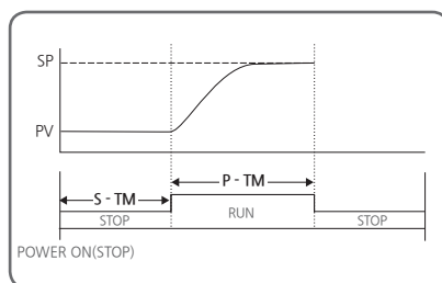
[Fig.16] S-TM Mode Operation
