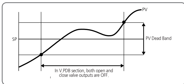
[Fig.25] V.P.DB (Valve PV Dead Band)
