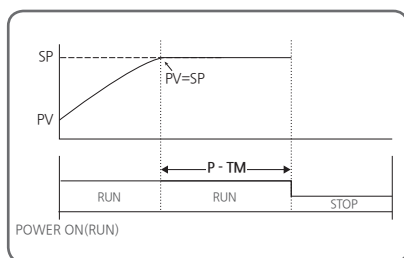
[Fig.15] PV=SP Mode Operation
