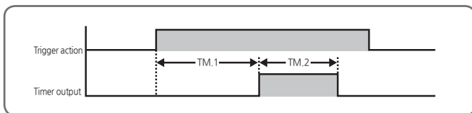
[Fig.35] Timer Delay 2
