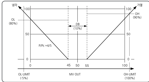
[Fig.12] Heating and Cooling under PID Control
