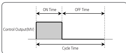
[Fig.40] Conditions for Detecting Heater Break Alarm
