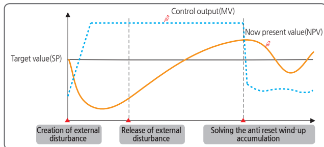
[Fig.5] When there is no anti reset wind-up (ARW) function
