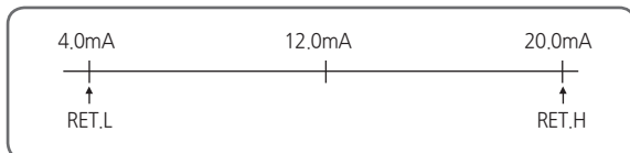
[Fig.42] In Case the Type of Retransmission is 'PV' or 'SP'
