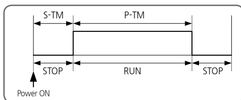
[Fig.17] Reservation Run Function
