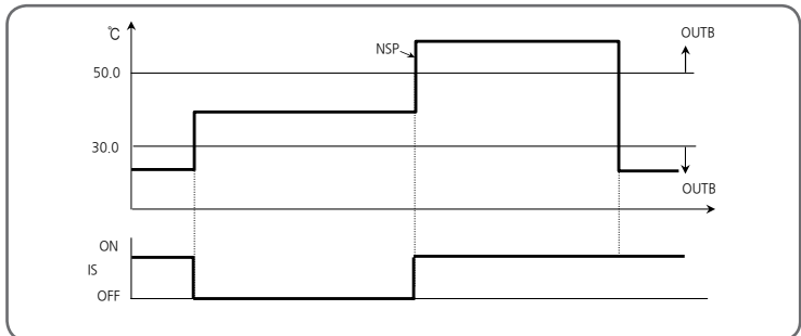
[Fig.31] Example of Inner Signal Case #2
