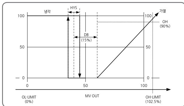
[Fig.14] Heating = PID Control, Cooling = ON / OFF
