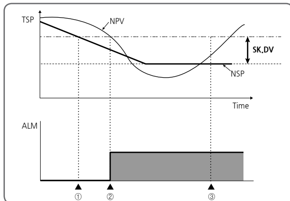
[Fig.29] DOWN SLOPE(∨ : SP ramping down)
