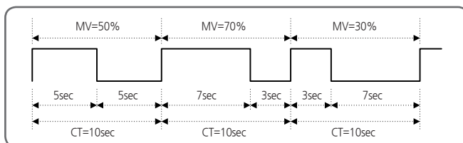
[Fig.22] In case the cycle time is 10 sec (CT = 10)
