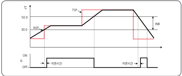
[Fig.32] Example of Inner Signal Case #3
