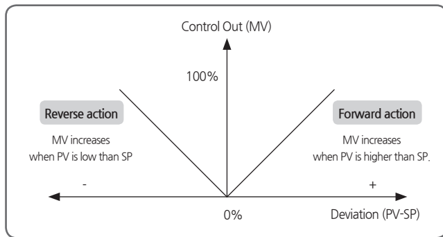
[Fig.21] Forward and Reverse Control Action
