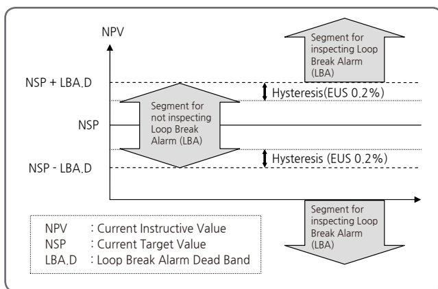
[Fig.41] Loop Break Alarm Dead Band
