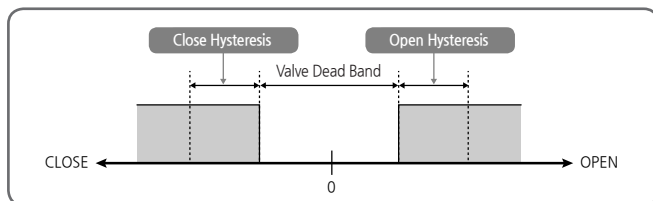
[Fig.24] V.DB and V.HYS Operation
