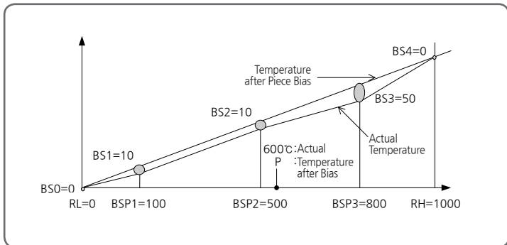
[Fig.19] Example of Piece Bias Formula
