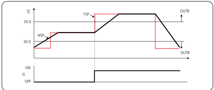
[Fig.33] Example of Inner Signal Case #4
