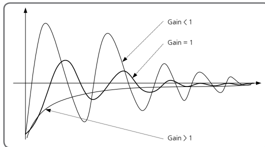
[Fig.3] Auto Tuning Gain(AT GAIN)
