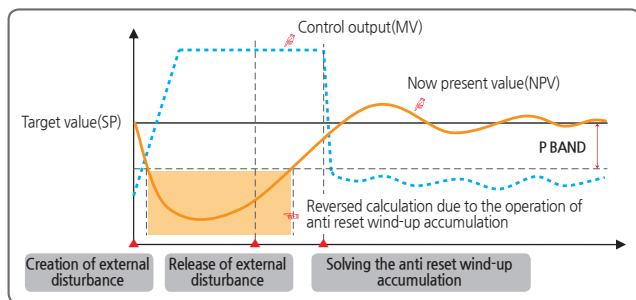
[Fig.6] When there is anti reset wind-up (ARW) function
