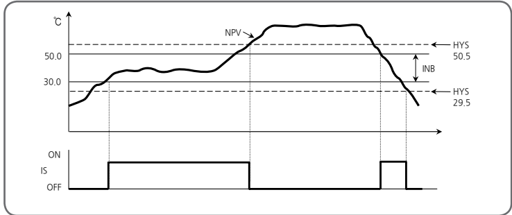
[Fig.30] Example of Inner Signal Case #1
