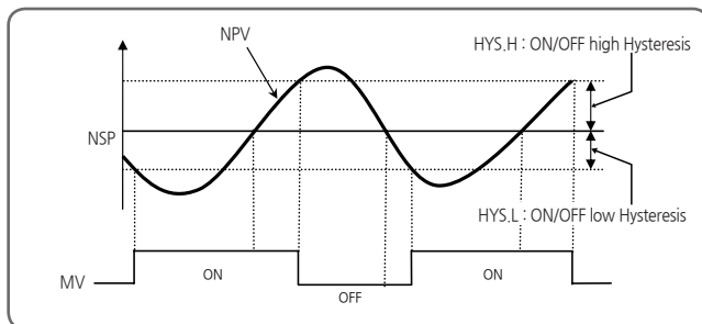
[Fig.26] ON/OFF Control
