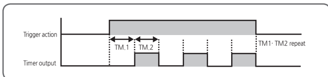
[Fig.36] Timer Flicker 1
