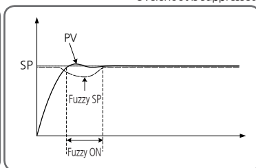
[Fig.11] Fuzzy ON
