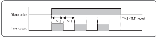
[Fig.37] Timer Flicker 2
