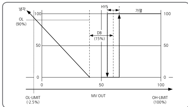
[Fig.13] Heating = ON / OFF, Cooling = PID Control
