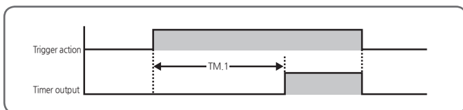
[Fig.34] Timer Delay 1
