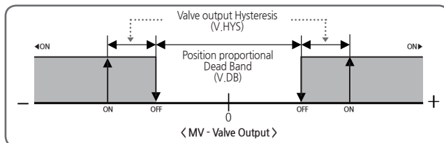
[Fig.23] Position proportional valve output operation
