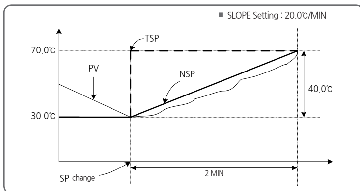
[Fig.4] Operation of SLOPE
