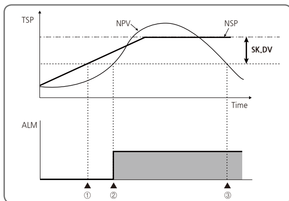
[图21] UP SLOPE(↗ : SP上升变化中)动作时
